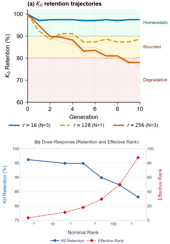
Figure 3: (a) K0 retention trajectories over 10 recursive generations for three representative ranks on Qwen 2.5 1.5B. Semi-transparent lines show individual seeds; solid thick lines show the per-rank mean. Background bands indicate regime classification (green: homeostatic, yellow: bounded, red: degradative). (b) Dose-response relationship: retention at last evaluated generation (Gen5 for r = 4, 32 ; Gen10 otherwise) versus nominal rank (left axis); mean effective rank versus nominal rank (right axis). Effective rank grows sub-linearly with nominal rank, indicating that increases in nominal capacity translate into progressively smaller increases in effective update dimensionality.
