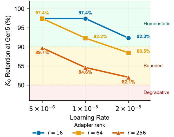
Figure 7: Rank \times learning-rate joint pattern on Qwen 2.5 1.5B (Gen5 retention). Descriptive non-parallel trends suggest that rank and learning rate may jointly determine the operating regime, but the single-seed design is hypothesis-generating rather than confirmatory.
