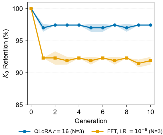
Figure 6: K_0 retention over 10 recursive generations for QLoRA r = 16 and FFT at LR = 10^{-6} on Qwen 2.5 1.5B. Lines show the mean across three seeds; shaded bands indicate 1 standard deviation.
