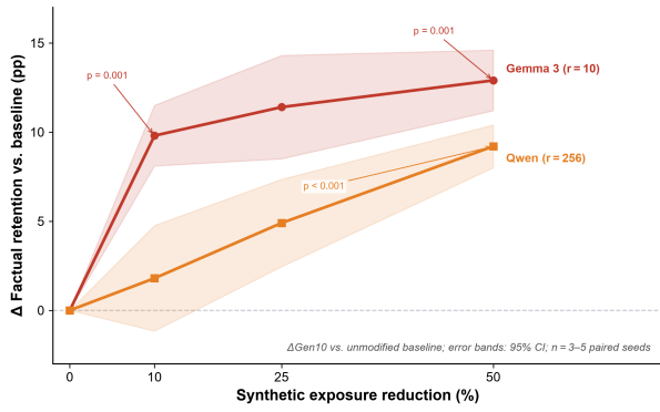
Figure 10: Dose–response of synthetic exposure reduction on factual retention across two backbones (Gen10, K_0 -conditioned). Each curve shows the mean improvement ( \Delta pp ) over the respective unmodified baseline as the fraction of synthetic training examples removed increases from 0% to 50%. Red circles: Gemma 3 1B at r = 10 ( n = 3 paired seeds; K_{0,G2} = 44 ). Orange squares: Qwen 2.5 1.5B at r = 256 ( n = 5 paired seeds; K_0 = 78 ). Shaded bands: 95 % confidence intervals from paired t -tests. The absolute gain is larger for Gemma 3 G2 ( K_{0,G2}=44 ) than for Qwen B7 ( K_0=78 ); effective rank is not portable across architectures, so the two curves are reported within their respective protocols rather than as a cross-backbone pressure comparison. Dashed horizontal line: no change ( \Delta = 0 pp).
