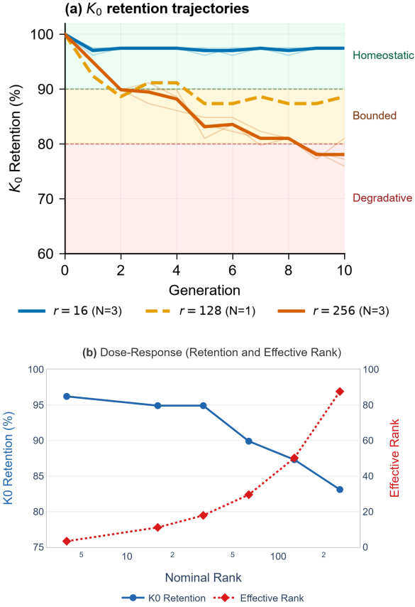
Figure 3: (a) Trajectories for the multi-seed runs ( r = 16 : N = 3 , G3 bf16; r = 256 : N = 3 , G1); the single-seed NF4 sweep values tabulated in Table 4 appear in panel (b). (a) K_0 retention trajectories over 10 recursive generations for three representative ranks on Qwen 2.5 1.5B. Semi-transparent lines show individual seeds; solid thick lines show the per-rank mean. Background bands indicate regime classification (green: homeostatic, yellow: bounded, red: degradative). (b) Dose-response relationship: retention at last evaluated generation (Gen5 for r = 4, 32 ; Gen10 otherwise) versus nominal rank (left axis); mean effective rank versus nominal rank (right axis). Effective rank grows sub-linearly with nominal rank, indicating that increases in nominal capacity translate into progressively smaller increases in effective update dimensionality.
