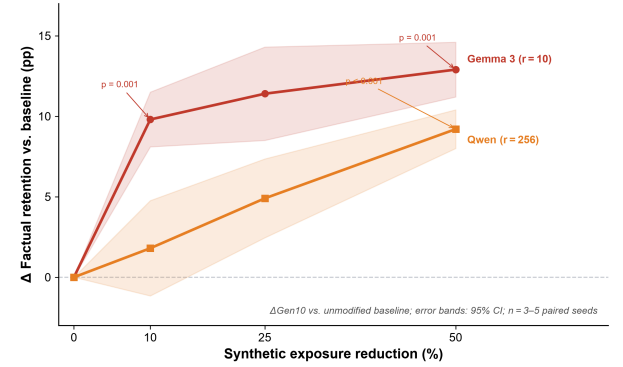
Figure 10: Dose-response of synthetic exposure reduction on factual retention across two backbones (Gen10, K_0 -conditioned). Each curve shows the mean improvement ( \Delta pp) over the respective unmodified baseline as the fraction of synthetic training examples removed increases from 0% to 50%. Red circles: Gemma 3 1B at r = 10 ( n = 3 paired seeds; K_{0,G2} = 44 ). Orange squares: Qwen 2.5 1.5B at r = 256 ( n = 5 paired seeds; K_0 = 78 ). Shaded bands: 95% confidence intervals from paired t -tests. The absolute gain is larger for Gemma 3 G2 ( K_{0,G2}=44 ) than for Qwen B7 ( K_0=78 ); effective rank is not portable across architectures, so the two curves are reported within their respective protocols rather than as a cross-backbone pressure comparison. Dashed horizontal line: no change ( \Delta = 0 pp).
