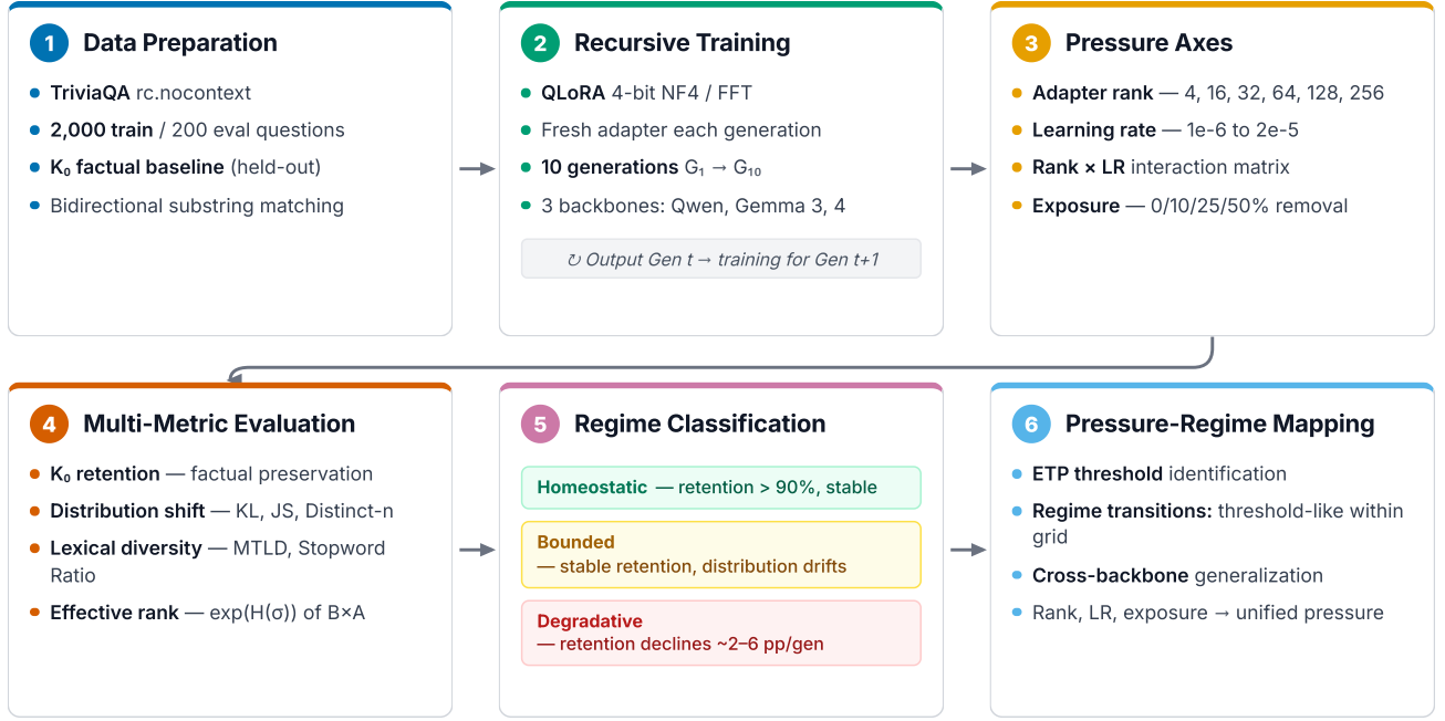
Figure 1: Overview of the experimental pipeline. (1) Data preparation and K_0 baseline establishment across three backbones (Qwen 2.5 1.5B, Gemma 3 1B, Gemma 4 E2B). (2) Recursive training over ten generations with strict data replacement. (3) Pressure manipulation along five axes: rank, learning rate, method, module topology, and synthetic-data dose (0/10/25/50% removal). (4) Per-generation evaluation of factual retention ( K_0 ), effective rank, response length, Distinct- n , MTLD, and stopword ratio. (5) Regime classification (Homeostatic, Bounded, Degradative). (6) Pressure-regime mapping: effective training pressure identified as the organizing principle for regime transitions.
