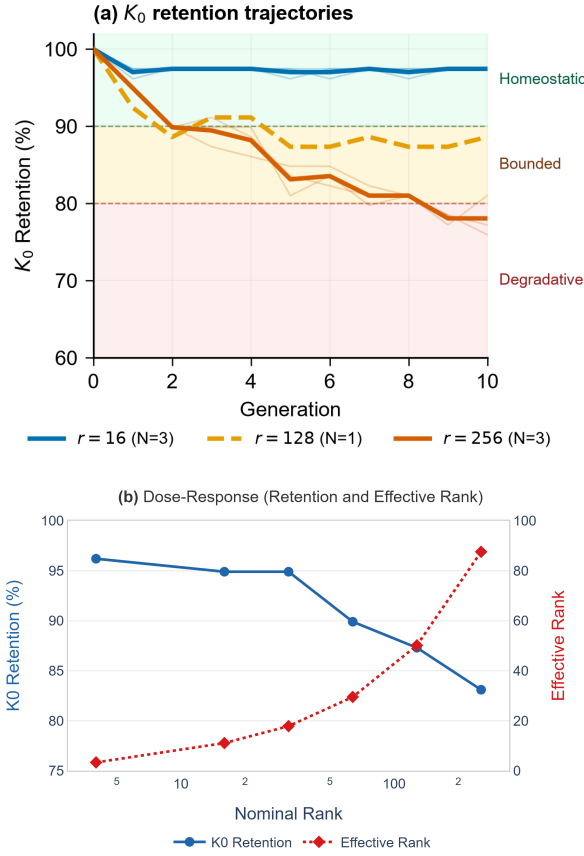
Figure 3: (a) K0 retention trajectories over 10 recursive generations for three representative ranks on Qwen 2.5 1.5B. Semi-transparent lines show individual seeds; solid thick lines show the per-rank mean. Background bands indicate regime classification (green: homeostatic, yellow: bounded, red: degradative). (b) Dose-response relationship: retention at last evaluated generation (Gen5 for r = 4, 32 ; Gen10 otherwise) versus nominal rank (left axis); mean effective rank versus nominal rank (right axis). Effective rank grows sub-linearly with nominal rank, indicating that increases in nominal capacity translate into progressively smaller increases in effective update dimensionality.
