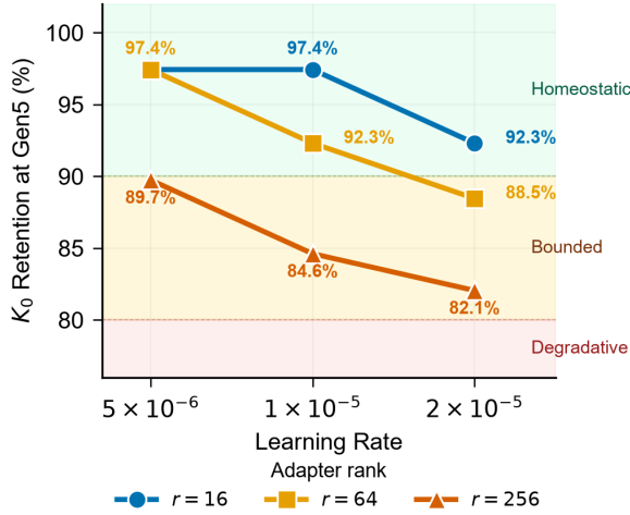
Figure 7: Rank & learning-rate joint pattern on Qwen 2.5 1.5B (Gen5 retention). Descriptive non-parallel trends suggest that rank and learning rate may jointly determine the operating regime, but the single-seed design is hypothesis-generating rather than confirmatory.
