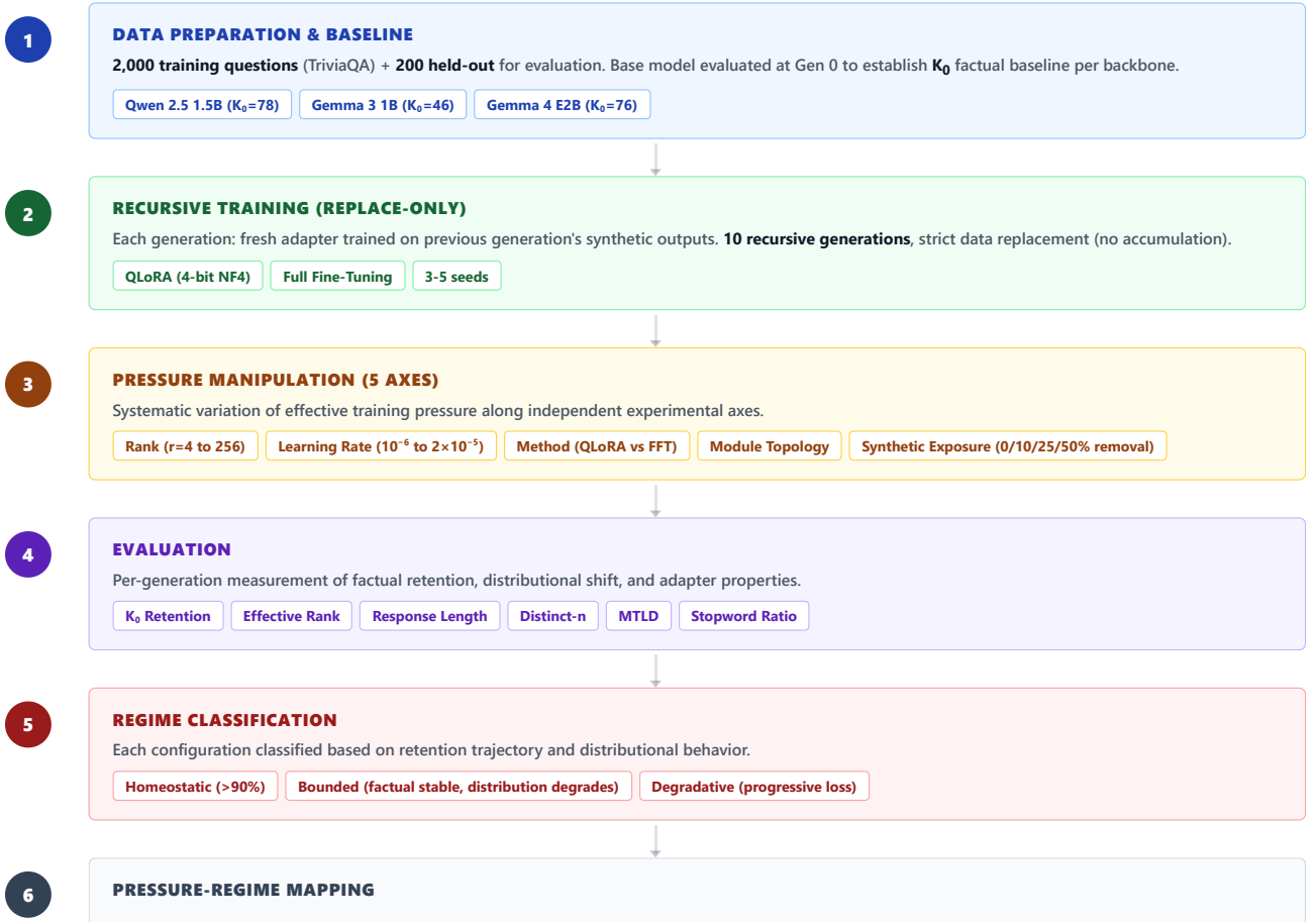
Figure 1: Overview of the experimental pipeline. (1) Data preparation and K_0 baseline establishment across three backbones (Qwen 2.5 1.5B, Gemma 3 1B, Gemma 4 E2B). (2) Recursive training over ten generations with strict data replacement. (3) Pressure manipulation along five axes: rank, learning rate, method, module topology, and synthetic-data dose (0/10/25/50% removal). (4) Per-generation evaluation of factual retention ( K_0 ), effective rank, response length, Distinct- n , MTLD, and stopword ratio. (5) Regime classification (Homeostatic, Bounded, Degradative). (6) Pressure-regime mapping: effective training pressure identified as the organizing principle for regime transitions.
