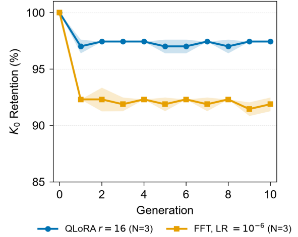
Figure 6: K_0 retention over 10 recursive generations for QLoRA r = 16 and FFT at LR = 10^{-6} on Qwen 2.5 1.5B. Lines show the mean across three seeds; shaded bands indicate \pm 1 standard deviation.
