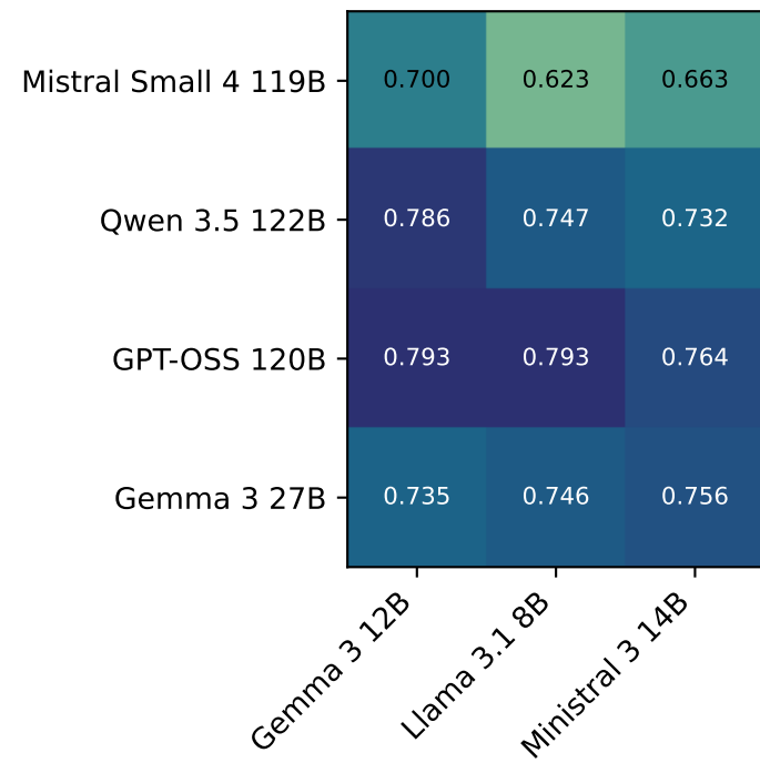
No Intent
