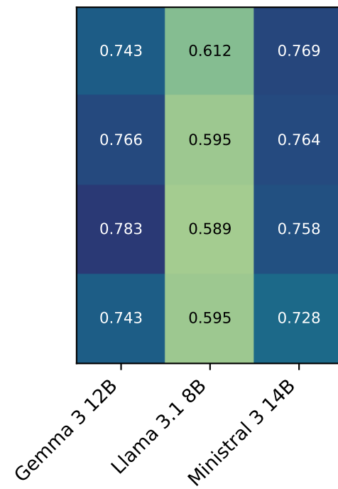
Human Intent
