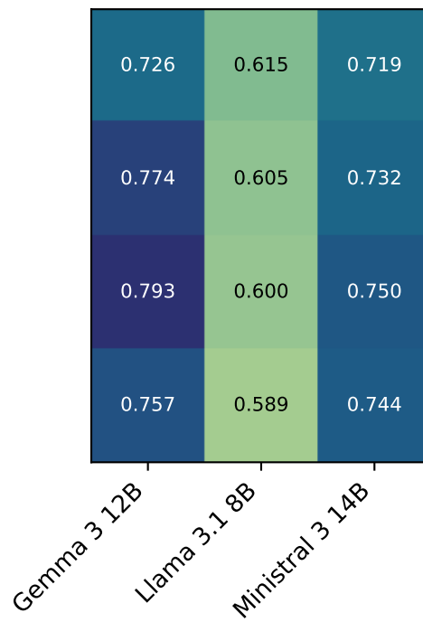
Synthetic Intent
