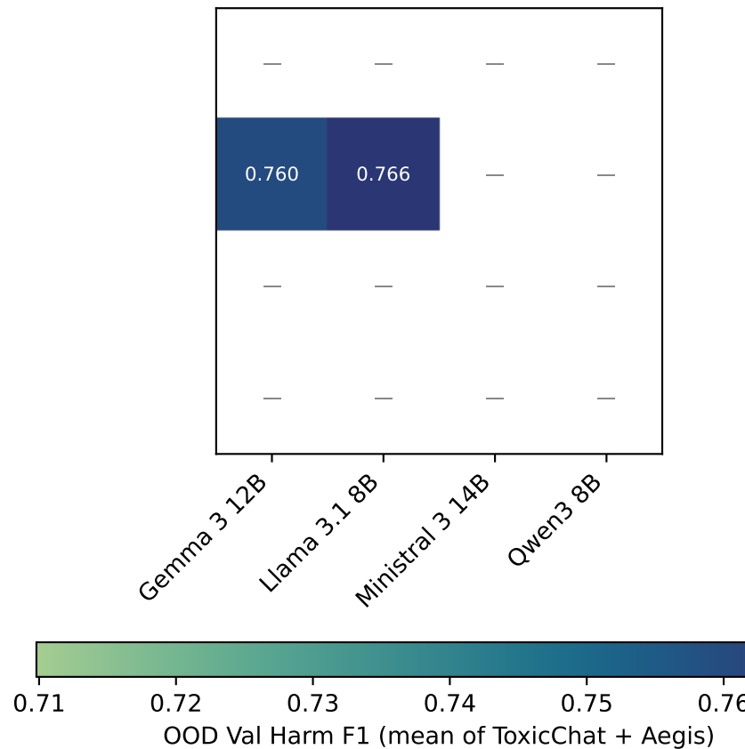
Synthetic Intent
