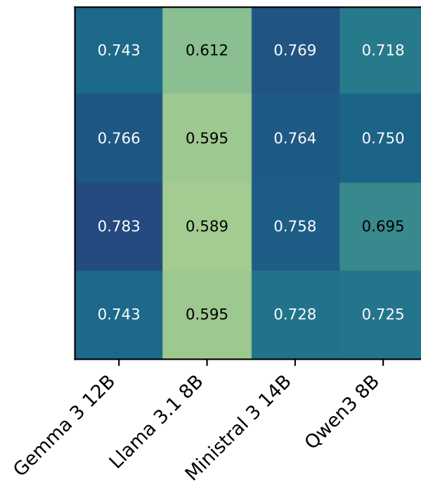
Human Intent
