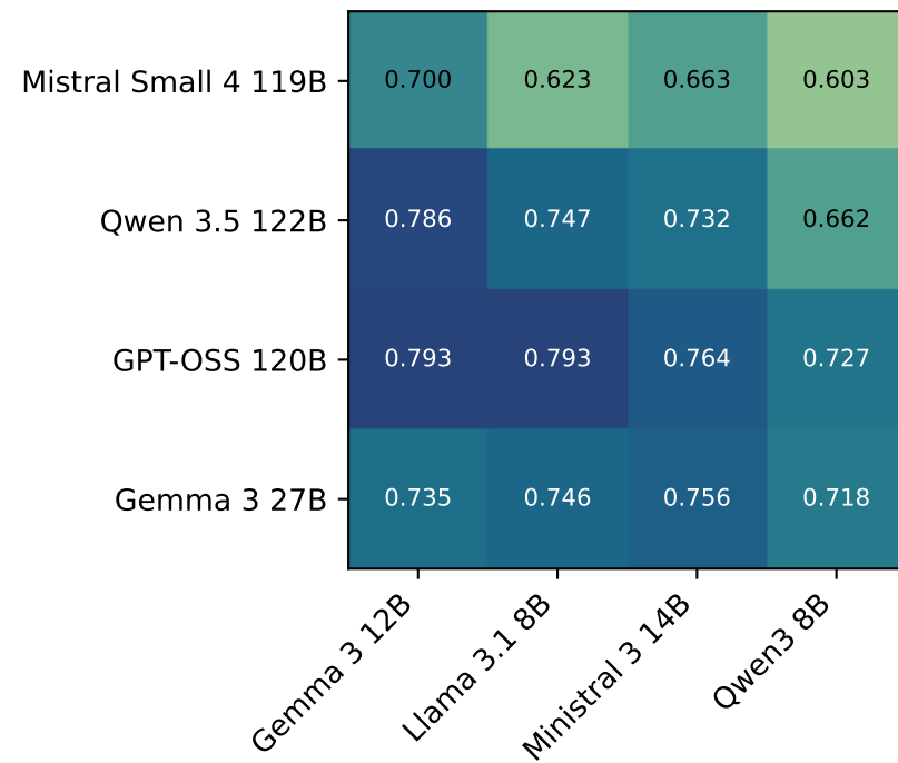
No Intent
