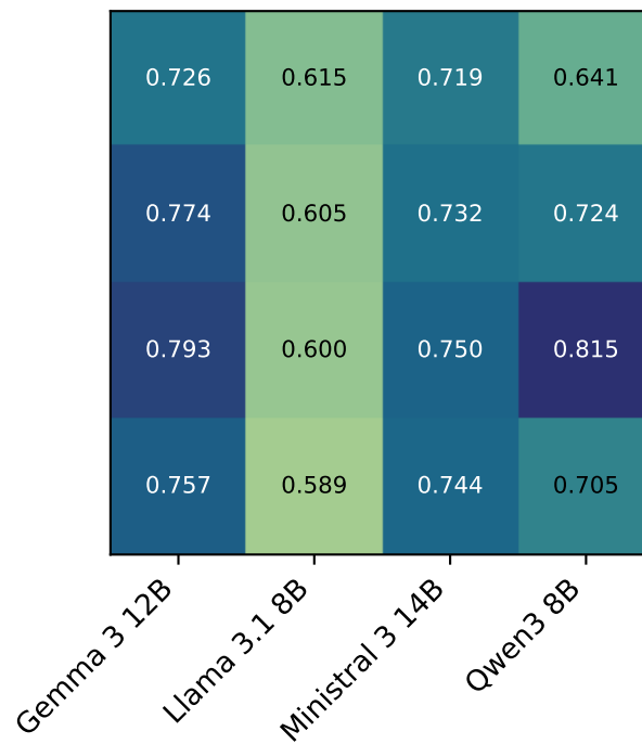
Synthetic Intent
