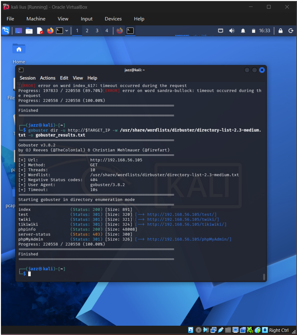
Figure 1 - Actual screenshot evidence: 06-gobuster-directory-results(M).png
