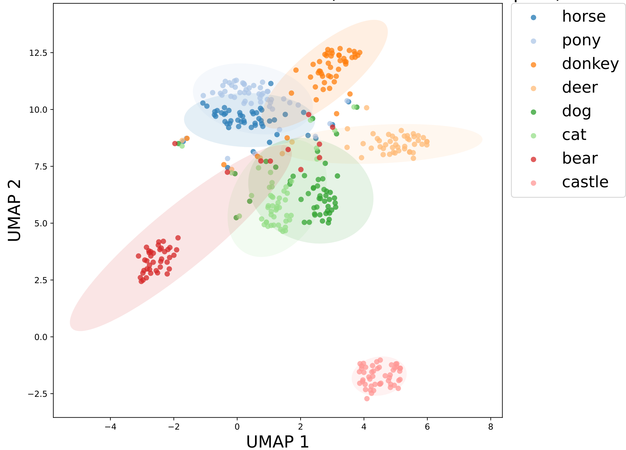
UMAP of Cross-Attention Activations (with covariance ellipses)
