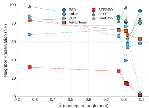
Figure 10: NP across concept entanglement levels for each unlearning method. Dashed lines connect concept-specific operating points from the same method in increasing order of \hat{\kappa} and are included as visual guides rather than fitted trends. Robust methods such as STEREO show a pronounced decline in NP as entanglement increases, while other methods exhibit weaker or more concept-dependent trends.
