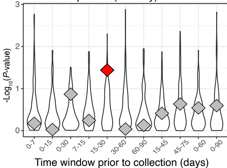
C Mean Precipitation (mm/day)
