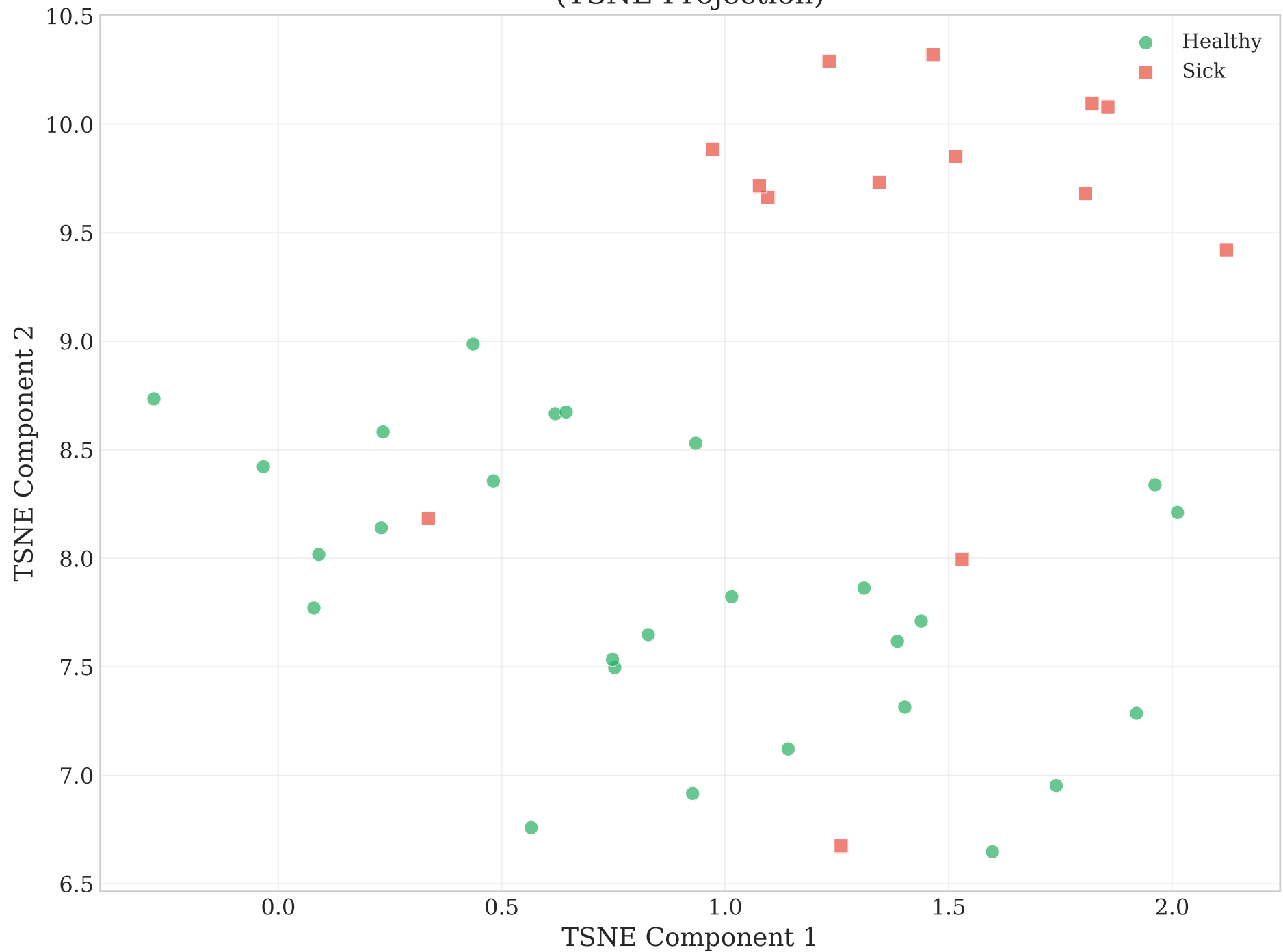
Feature Distribution - EfficientNet-B0 (TSNE Projection)
