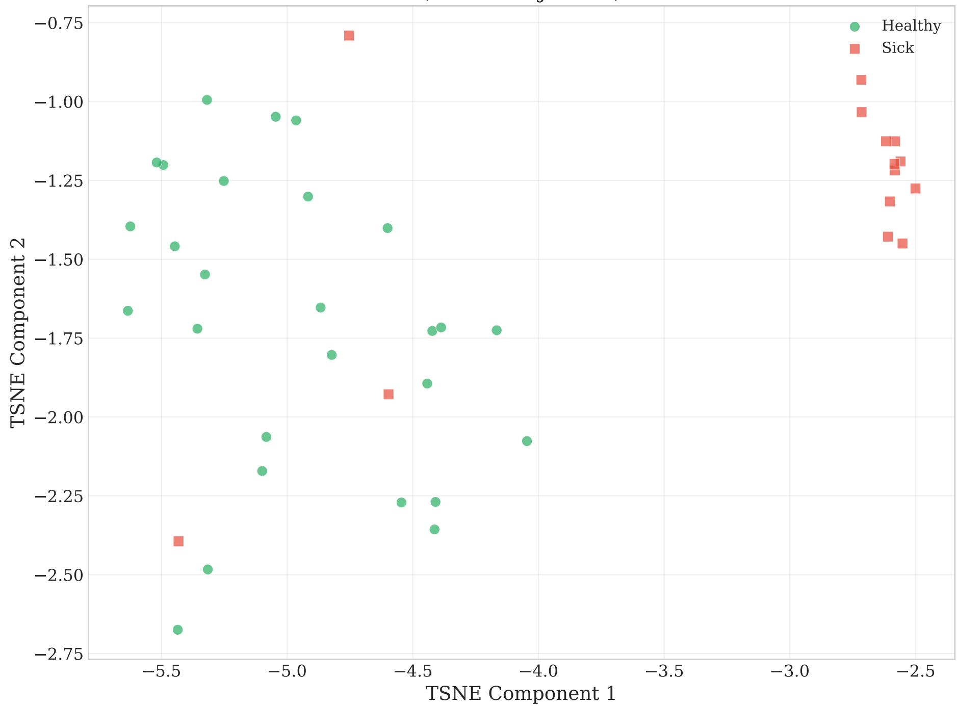
Feature Distribution - ResNet50 (TSNE Projection)
