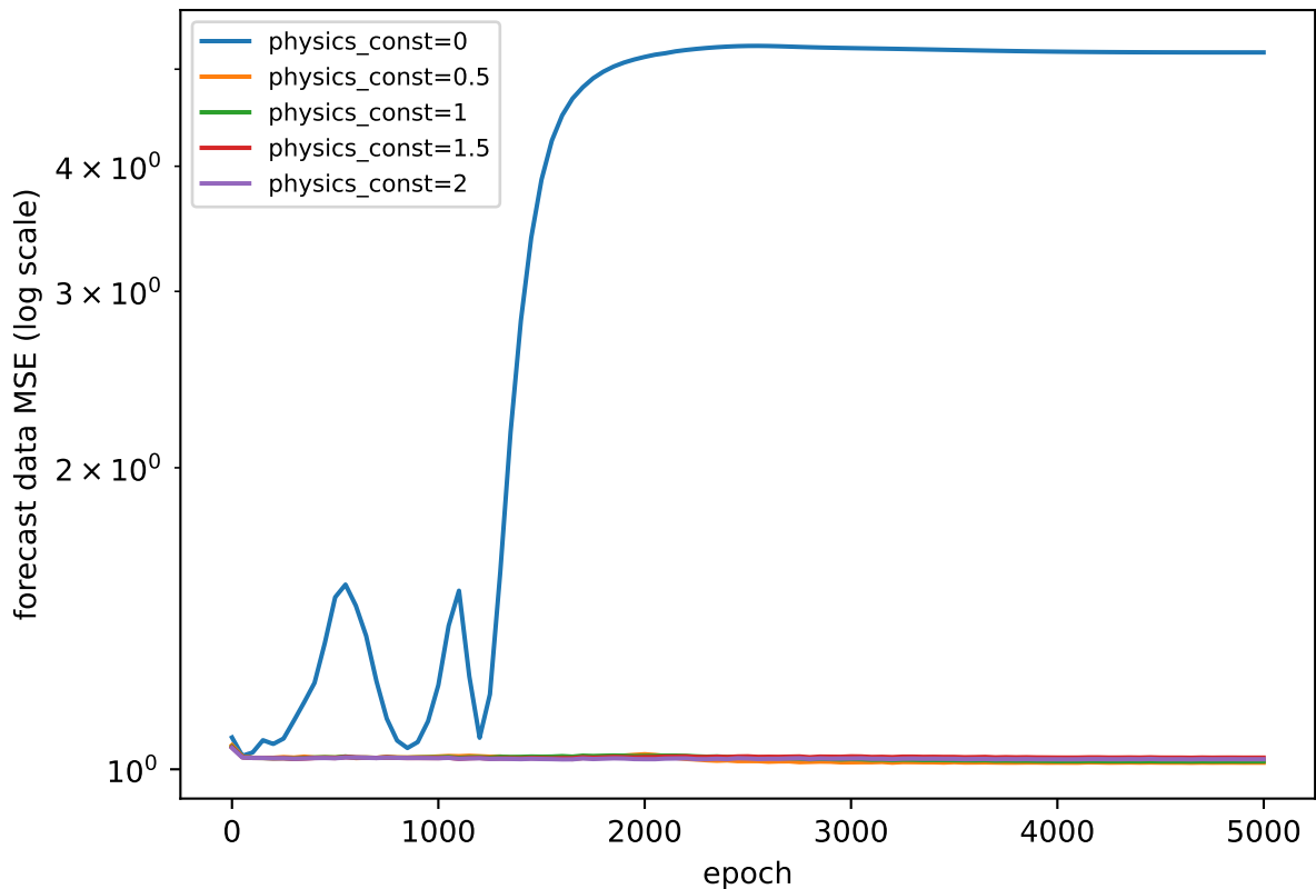
PINN forecast loss vs epoch — varying physics_const (defaults: {'hidden_neurons': 64, 'lr': 0.001, 'use_scheduler': True, 'n_colloc': 10000})
