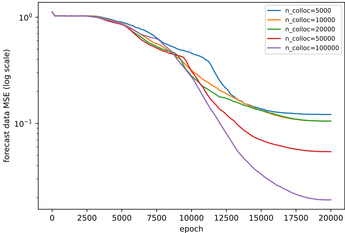
PINN forecast loss vs epoch — varying n_{\text{colloc}} (defaults: {'hidden_neurons': 256, 'lr': 0.001, 'use_scheduler': True, 'physics_const': 1.0})
