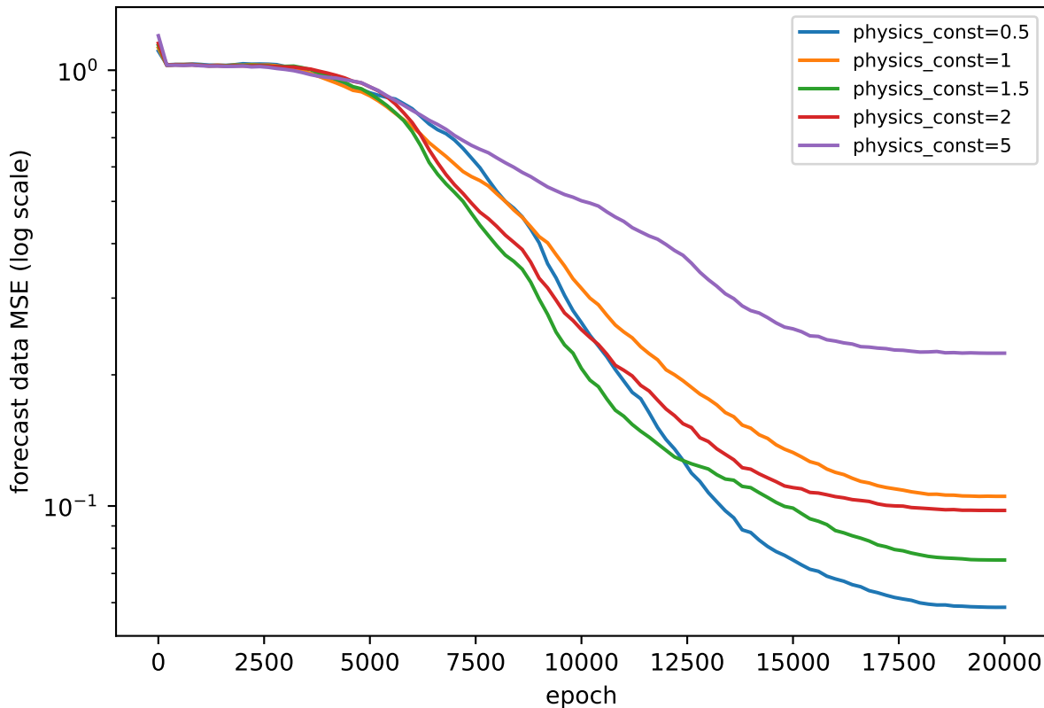
PINN forecast loss vs epoch — varying physics_const (defaults: {'hidden_neurons': 256, 'lr': 0.001, 'use_scheduler': True, 'n_colloc': 10000})
