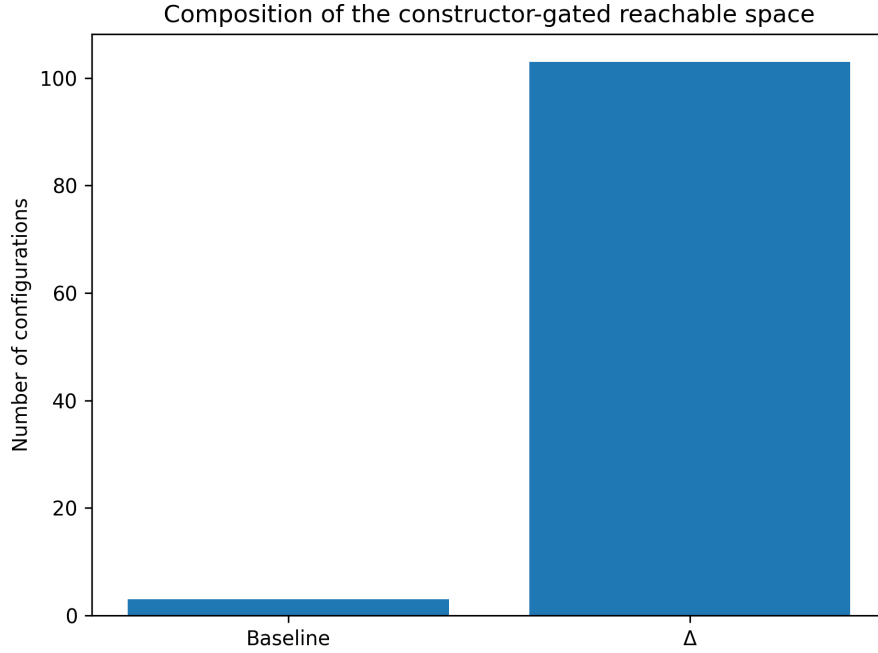
Figure 6: Dominance of the constructor-gated reachability expansion \Delta
