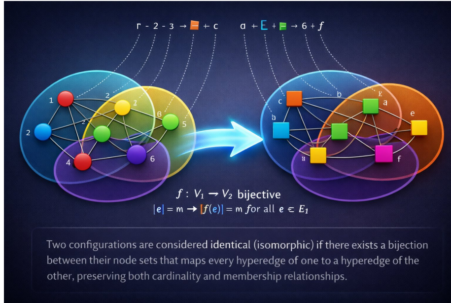
Figure 2: Example of isomorphic hypergraph configurations under canonicalization
