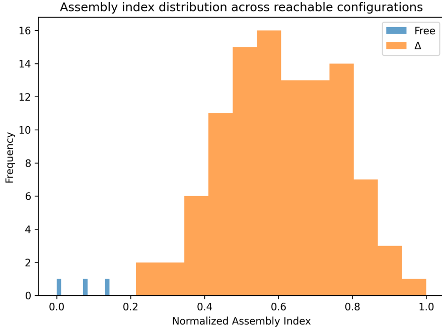
Figure 5: Assembly index distribution across reachable configurations
