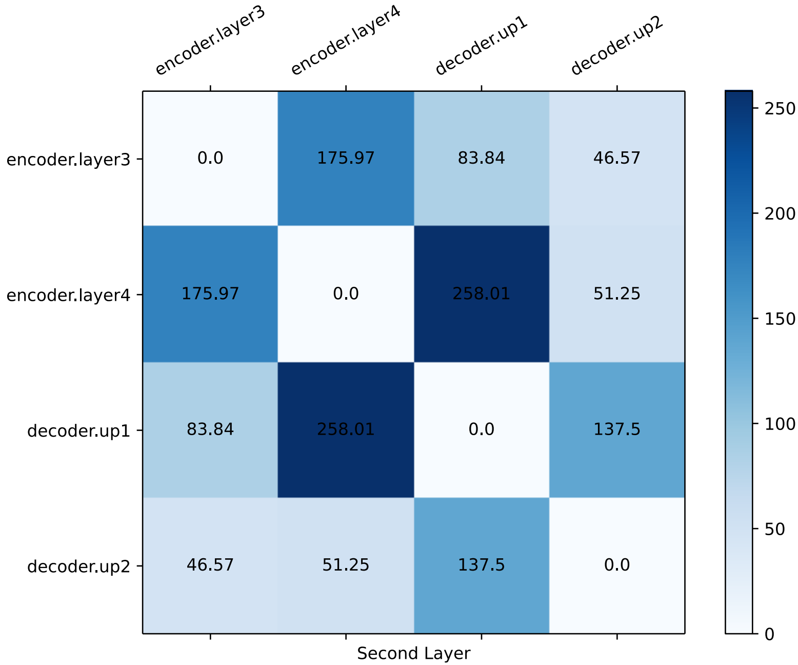
Area under curve for the prototype overlap per layer pair
