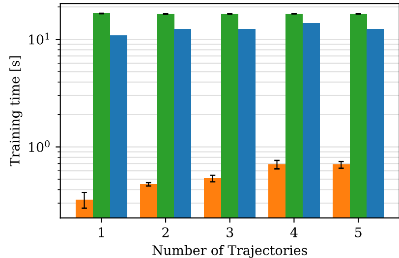
Single pendulum
