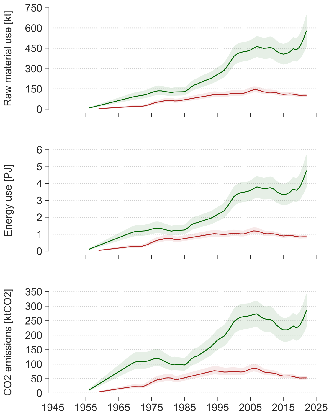
(b) Total flows of raw materials, energy and CO2
