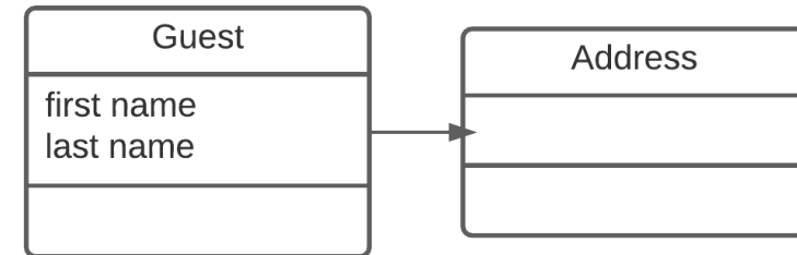
Domain model
