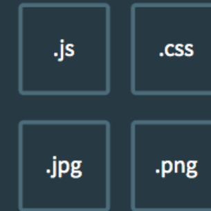
STATIC ASSETS
