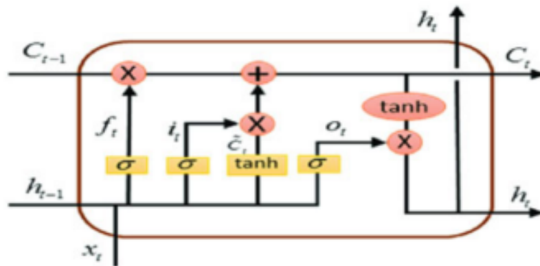
Figura 2.8: Arquitectura LSTM
