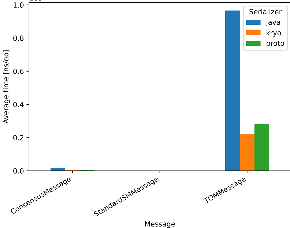
performance by message type
