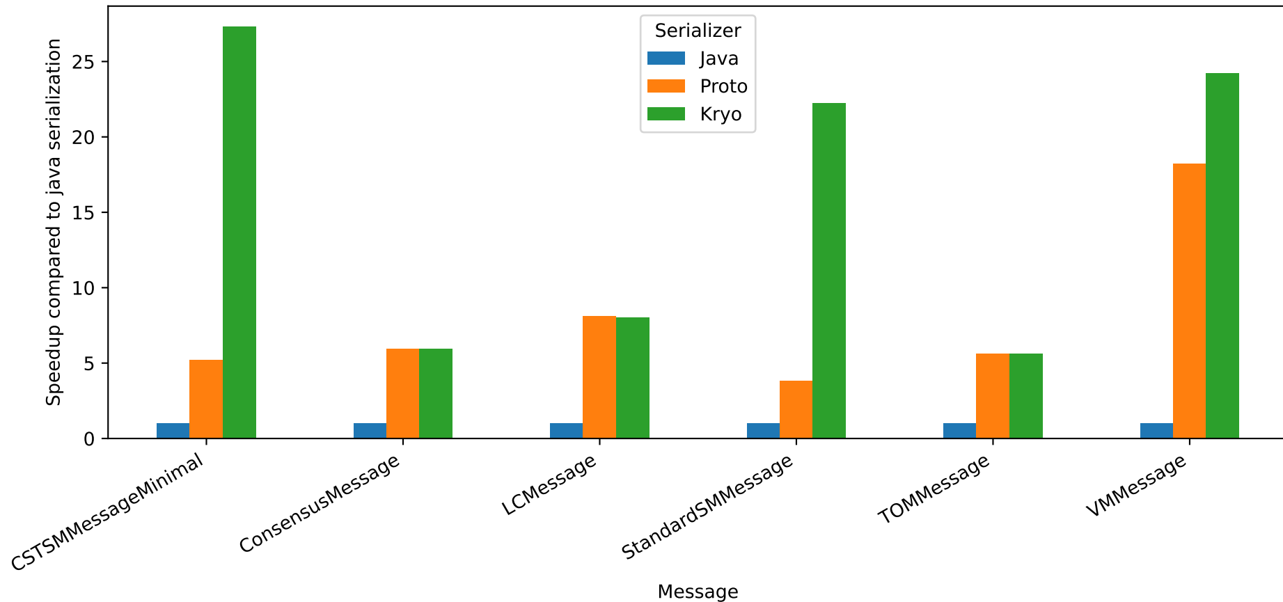
Relative speedup deserialize by message type
