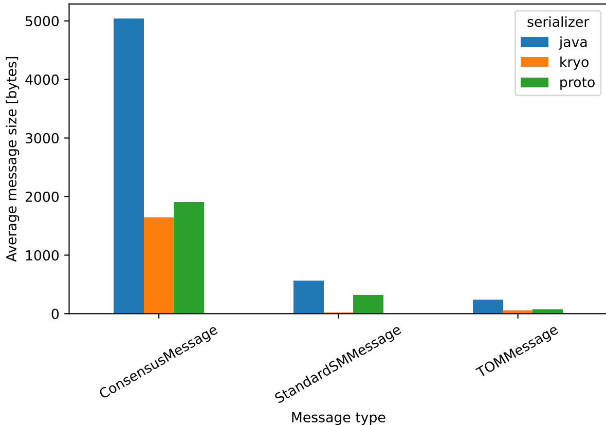
Average message size by serializer
