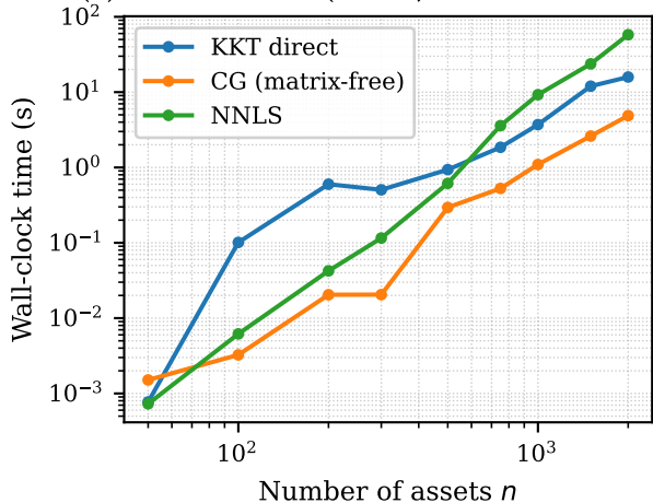
(a) Runtime vs. n ( T = 2n , with LW shrinkage)
