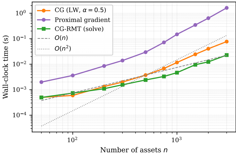
Runtime vs. n ( T = 1250 fixed)
