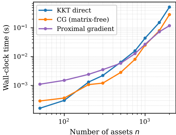
(a) Runtime vs. n ( T = 2n , LW shrinkage)
