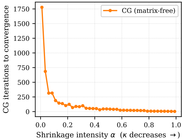
(b) Iterations vs. \alpha ( n = 500 , T = 250 )
