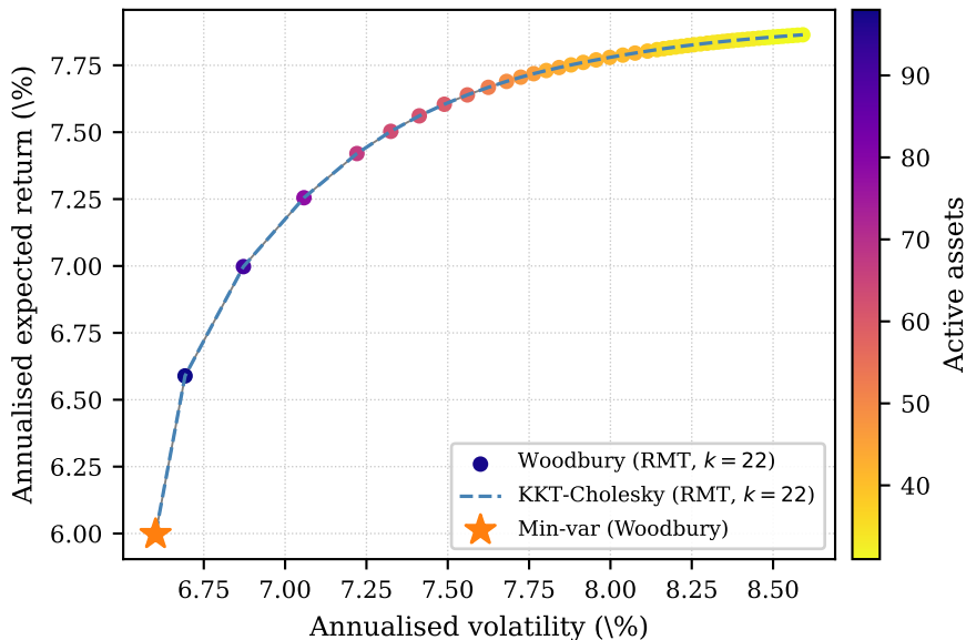
Efficient frontier ( n = 500 , T = 1250 , RMT k = 22 )
