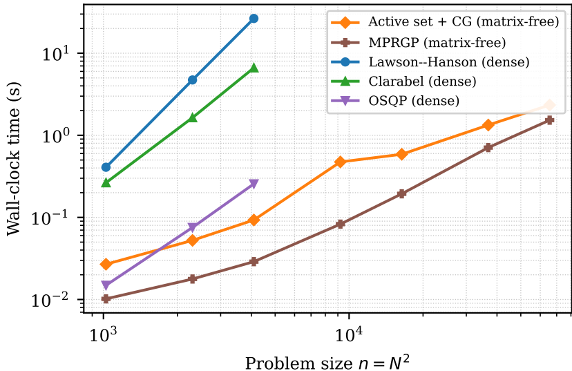
Matrix-free deblurring vs dense baselines
