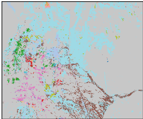
dominant endmember per pixel
