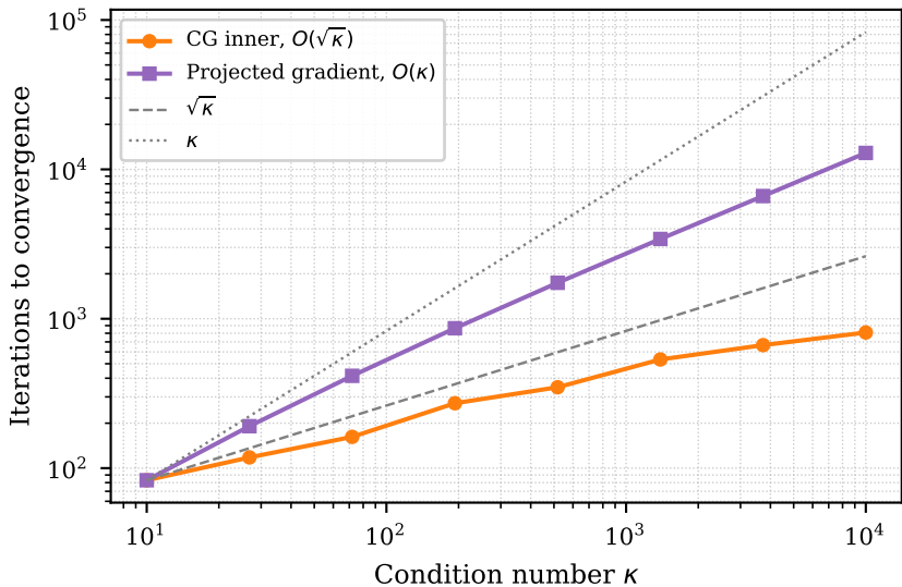
Krylov vs. first order ( n = 120 )
