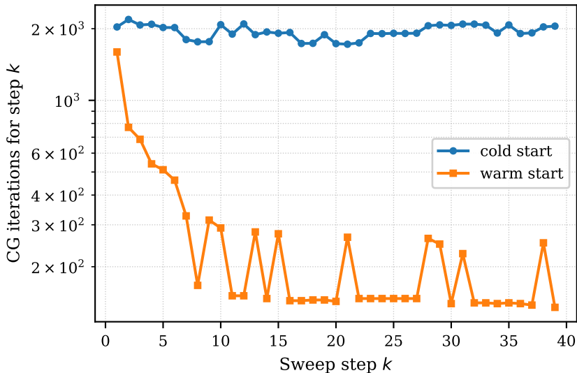
Warm-started sweep ( n = 200 , \kappa = 10^4 )
