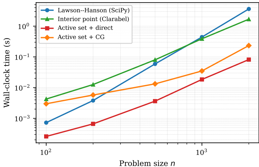
Solver comparison ( \kappa = 10^4 )
