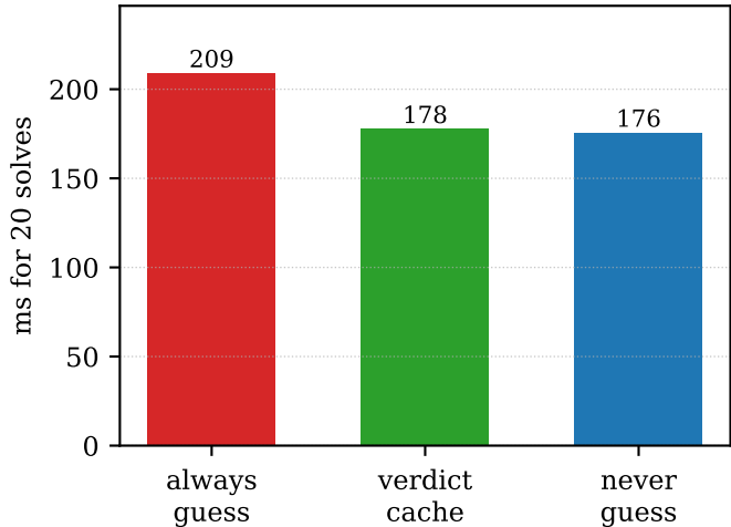
A family sharing an ill-conditioned G ( n = 400 , \kappa(T) = 10^6 )
