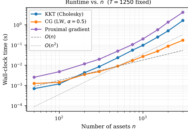
Figure 2: Wall-clock time vs number of assets n (log-log scale, T = 1250 fixed) for CG with LW shrinkage ( \alpha = 0.5 ), the dense KKT (Cholesky) baseline, and the proximal-gradient baseline. Data are generated from a latent factor model. Reference slopes O(n) and O(n^2) are anchored to the CG-LW curve at n = 500 ; CG-LW tracks well below O(n^2) and pulls steadily ahead of the dense KKT baseline as n grows, while proximal gradient tracks closer to O(n^2) as its O(\kappa) iteration count grows with the condition number.
