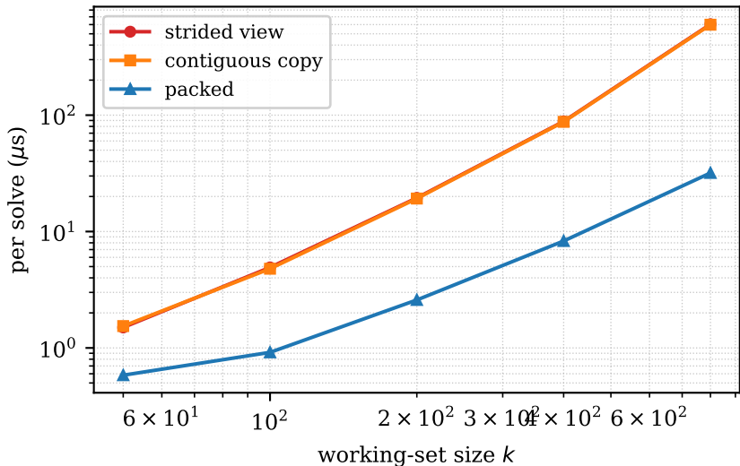
One triangular solve, three call shapes
