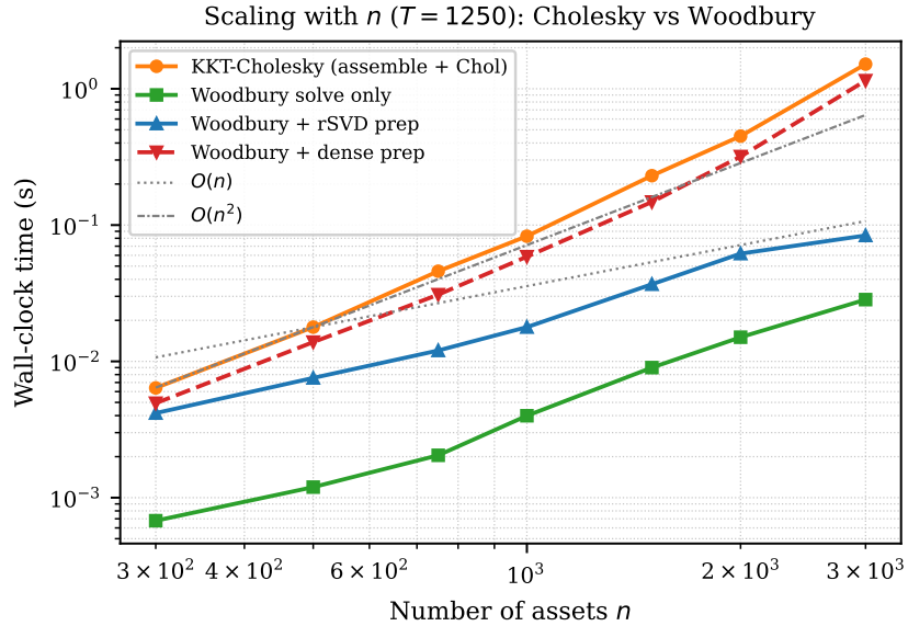
Figure 1: Wall-clock time vs. n (log-log, T = 1250 ; k grows as \approx n/24 ). KKT-Cholesky grows faster than Woodbury as n_a grows with n and the O(n_a^3) term dominates; dashed reference lines O(n) , O(n^2) anchored at n = 500 . At n = 3000 ( k = 125 ) the Woodbury solve is 53\times faster than KKT-Cholesky, and the full rSVD-plus-Woodbury pipeline (0.084 s) is 18\times faster than KKT-Cholesky (1.52 s), which is charged no preprocessing.
