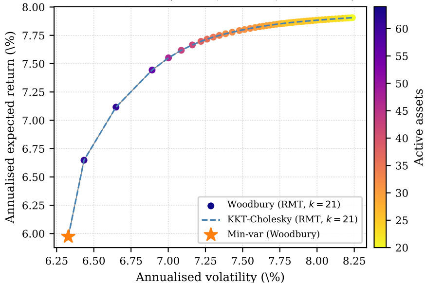
Efficient frontier ( n = 500 , T = 1250 , RMT k = 21 )
