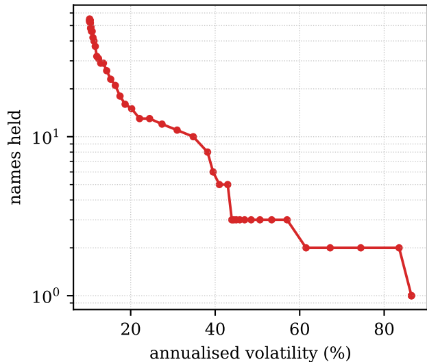
Holdings along the frontier
