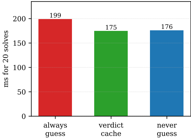
A family sharing an ill-conditioned G ( n = 400 , \kappa(T) = 10^6 )
