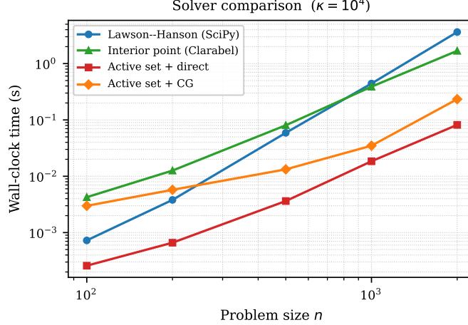
Figure 5: Wall-clock time against problem size n on the planted family ( \kappa = 10^4 , support 50%, mean over seeds): SciPy’s Lawson–Hanson NNLS and the Clarabel interior-point solver against Algorithm 1 with direct and matrix-free CG inner solves.
