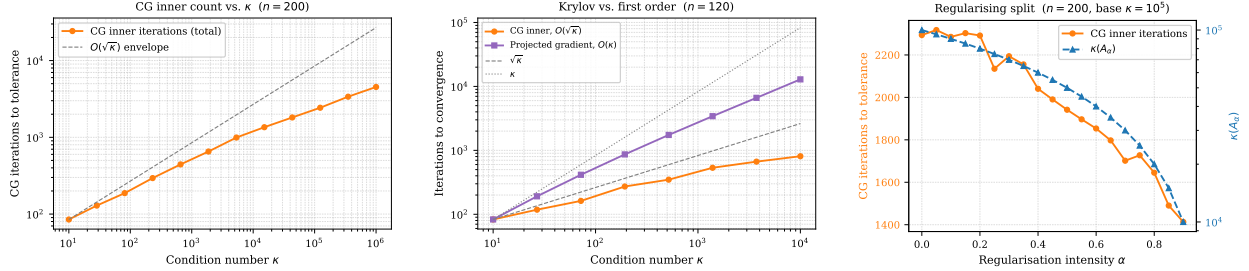
Figure 1: CG inner count vs. \kappa , Figure 2: Krylov vs. first order: Figure 3: Regularising split: under the O(\sqrt{\kappa}) envelope. O(\sqrt{\kappa}) vs. O(\kappa) . count falls as \kappa(A_\alpha) shrinks.
