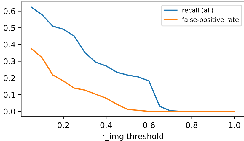
Threshold sweep
