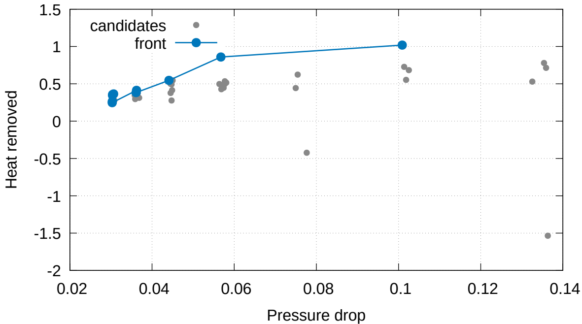
Channel fin Pareto front
