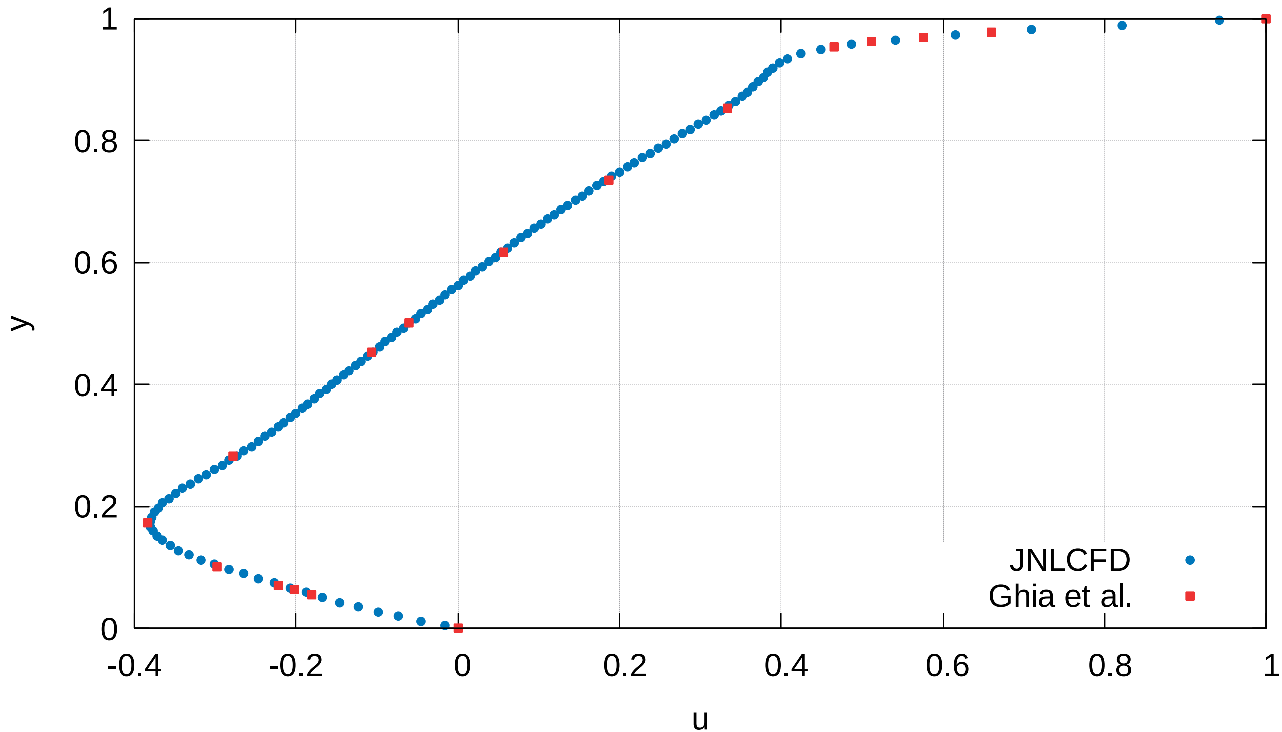
Lid-driven cavity: u at x=0.5, Re=1000
