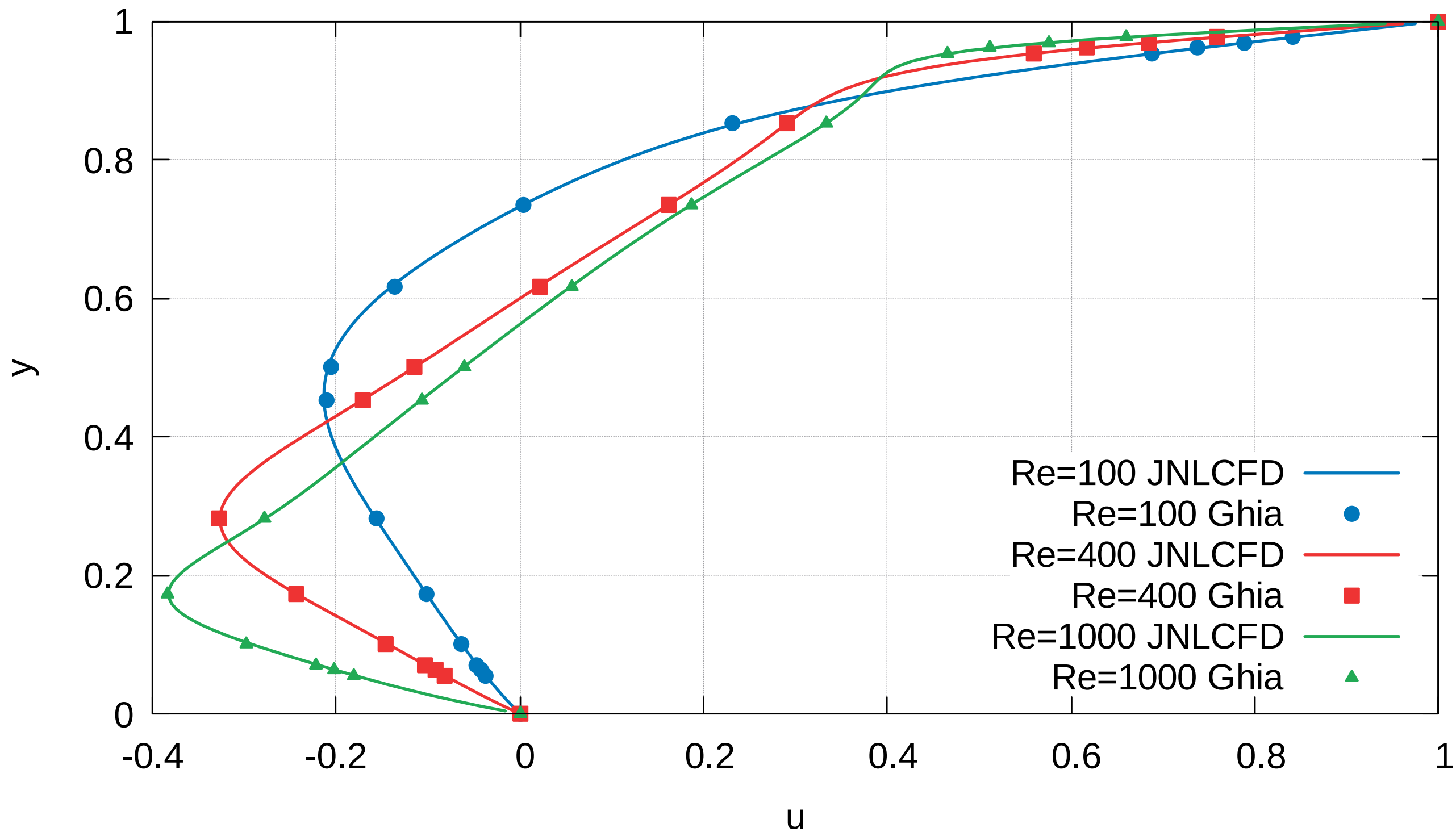
Lid-driven cavity: u at x=0.5 — Ghia et al. validation
