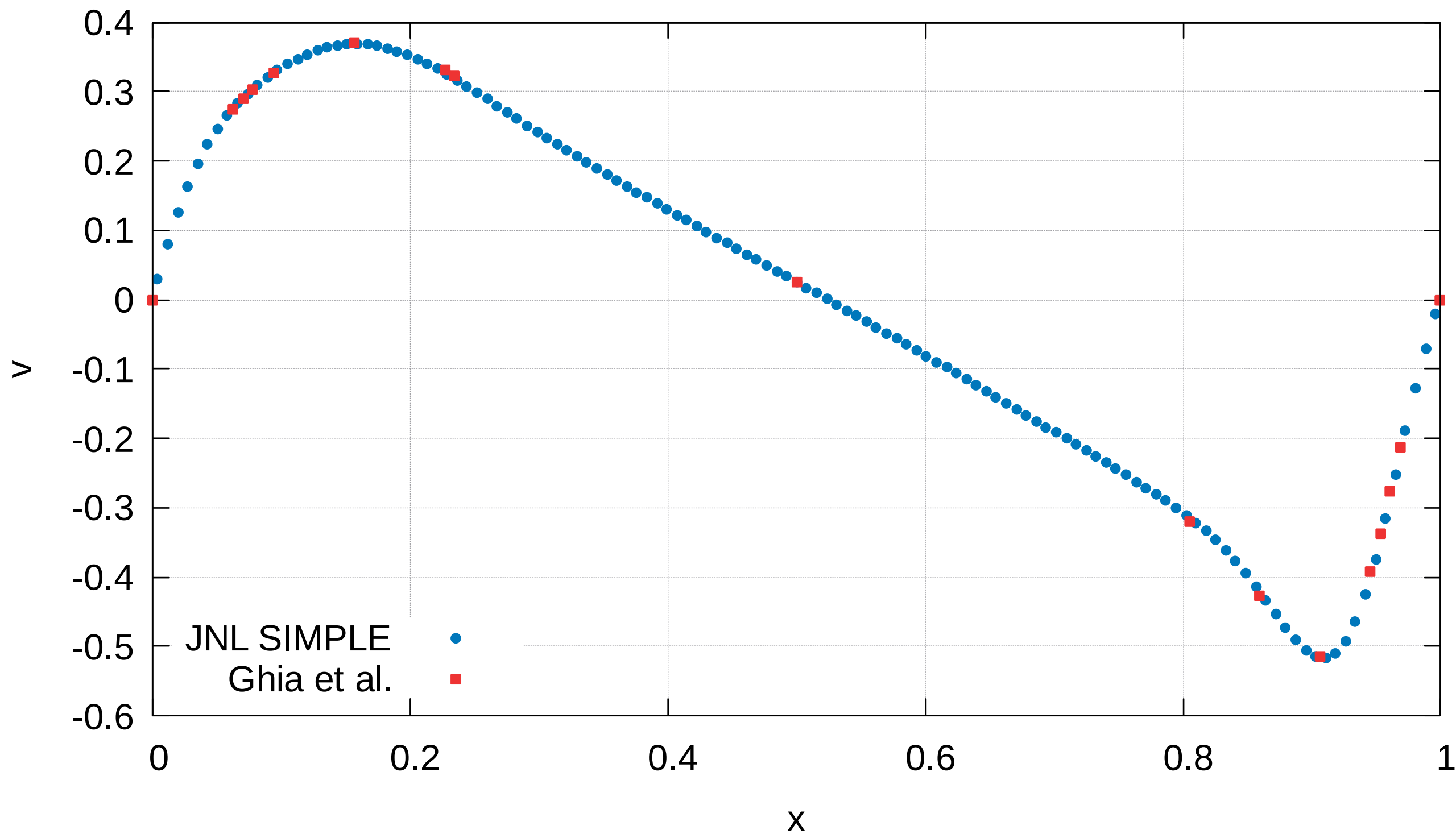
Lid-driven cavity: v at y=0.5 , Re=1000
